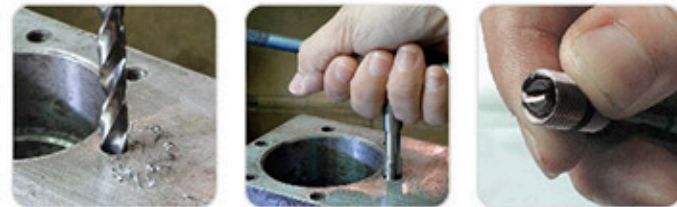
1. Drill out damaged thread using correctly sized drill bit 2. Tap re-drilled hole using tap 3. Load coiled insert into applicator
