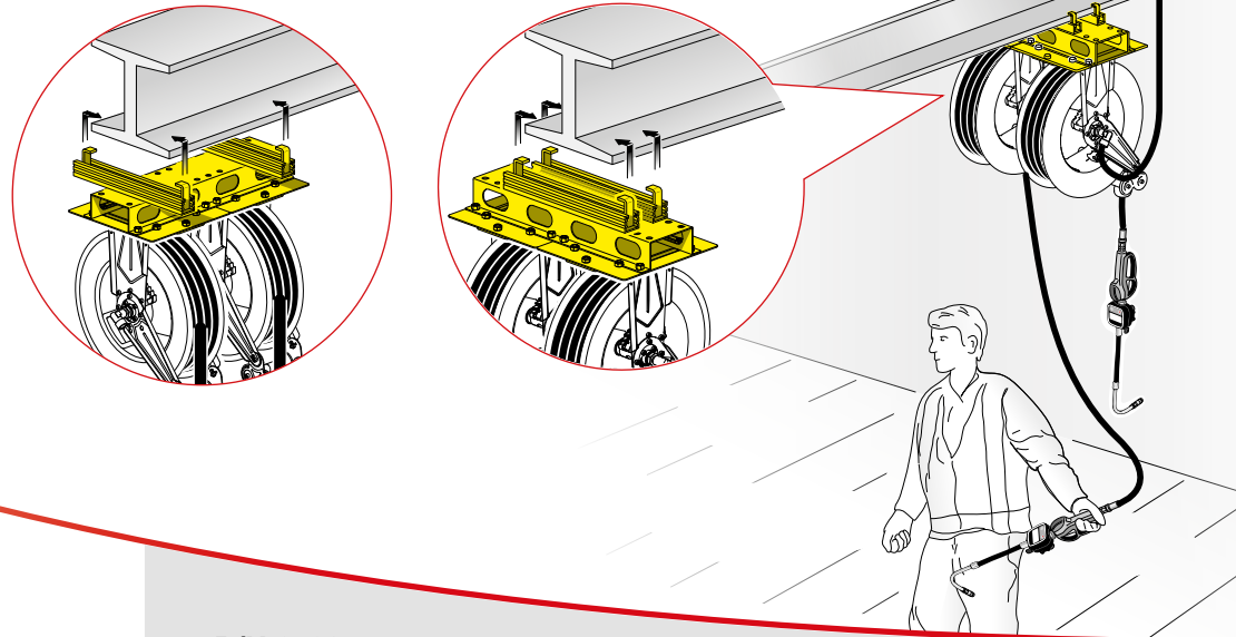
P/N 843011 Bracket for installing 1 hose reel s. 390 or 430 on HEA beam.
